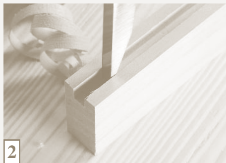
2 Here you can see the advantage of tool slaving. My chisel drops into the groove. The walls will guide the chisel.
