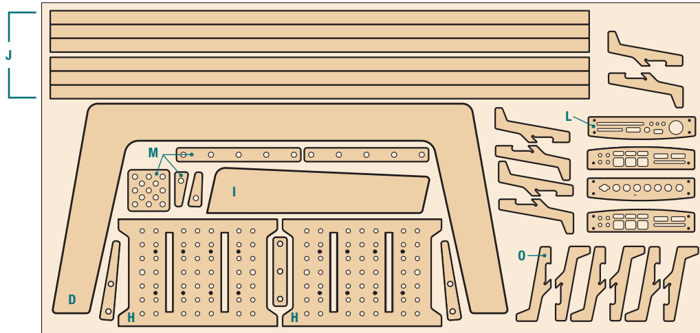
PLYWOOD LAYOUT 3
