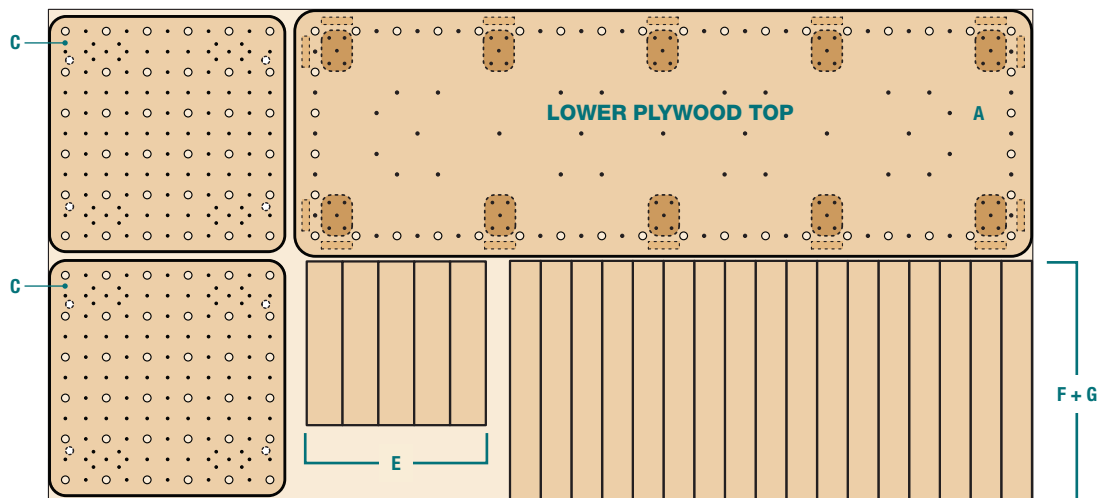
PLYWOOD LAYOUT 2
